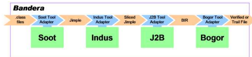
Fig. 1. Bandera Tool Framework Architecture
